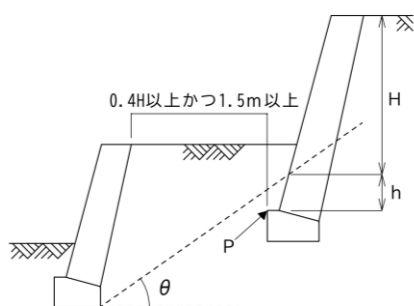
(a) 練積み造+練積み造
